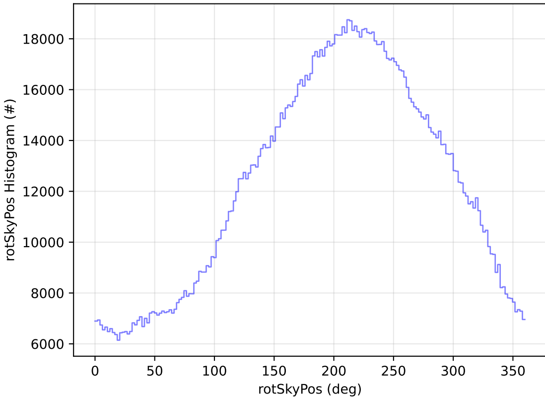
too_elab_r128_d3_ugrizy_v3.4_10yrs All sky all bands: rotSkyPos Histogram
