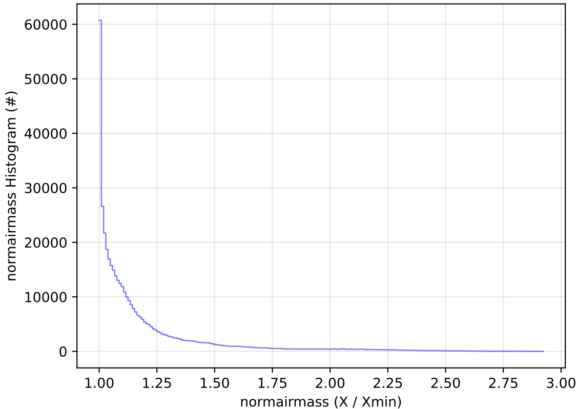
too_elab_r128_d3_ugrizy_v3.4_10yrs WFD z band: normairmass Histogram
