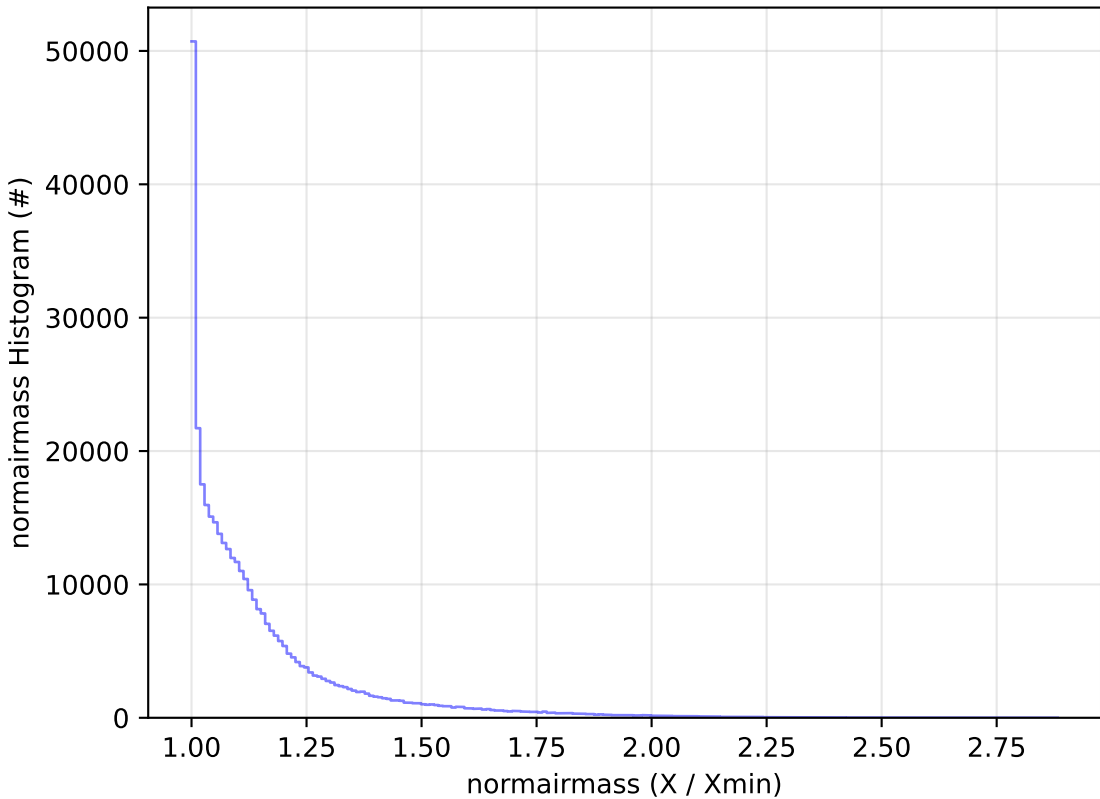
too_elab_r128_d3_ugrizy_v3.4_10yrs WFD y band: normairmass Histogram
