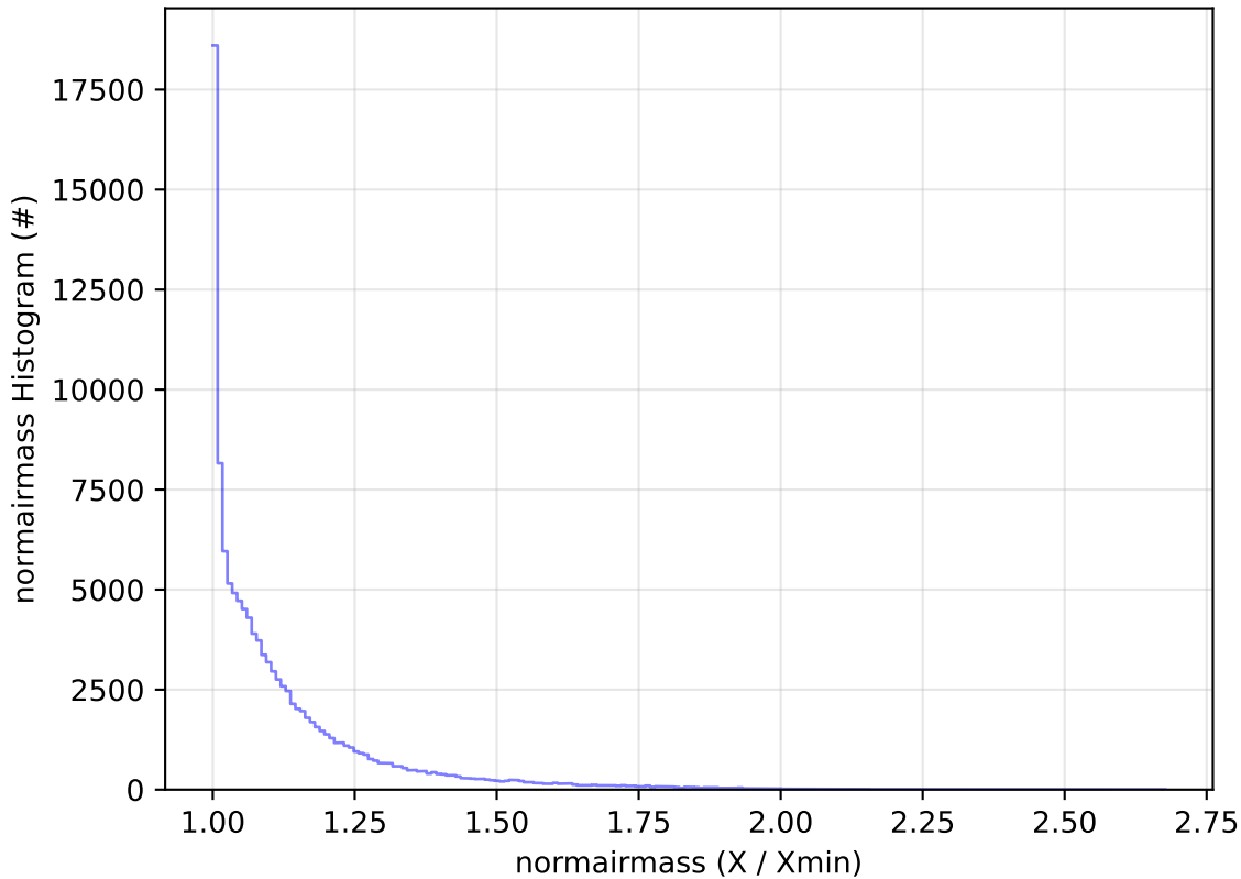
too_elab_r128_d3_ugrizy_v3.4_10yrs WFD u band: normairmass Histogram
