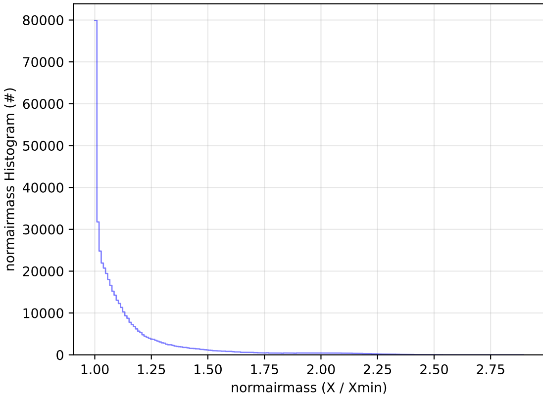
too_elab_r128_d3_ugrizy_v3.4_10yrs WFD r band: normairmass Histogram
