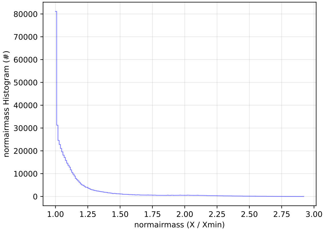
too_elab_r128_d3_ugrizy_v3.4_10yrs WFD i band: normairmass Histogram
