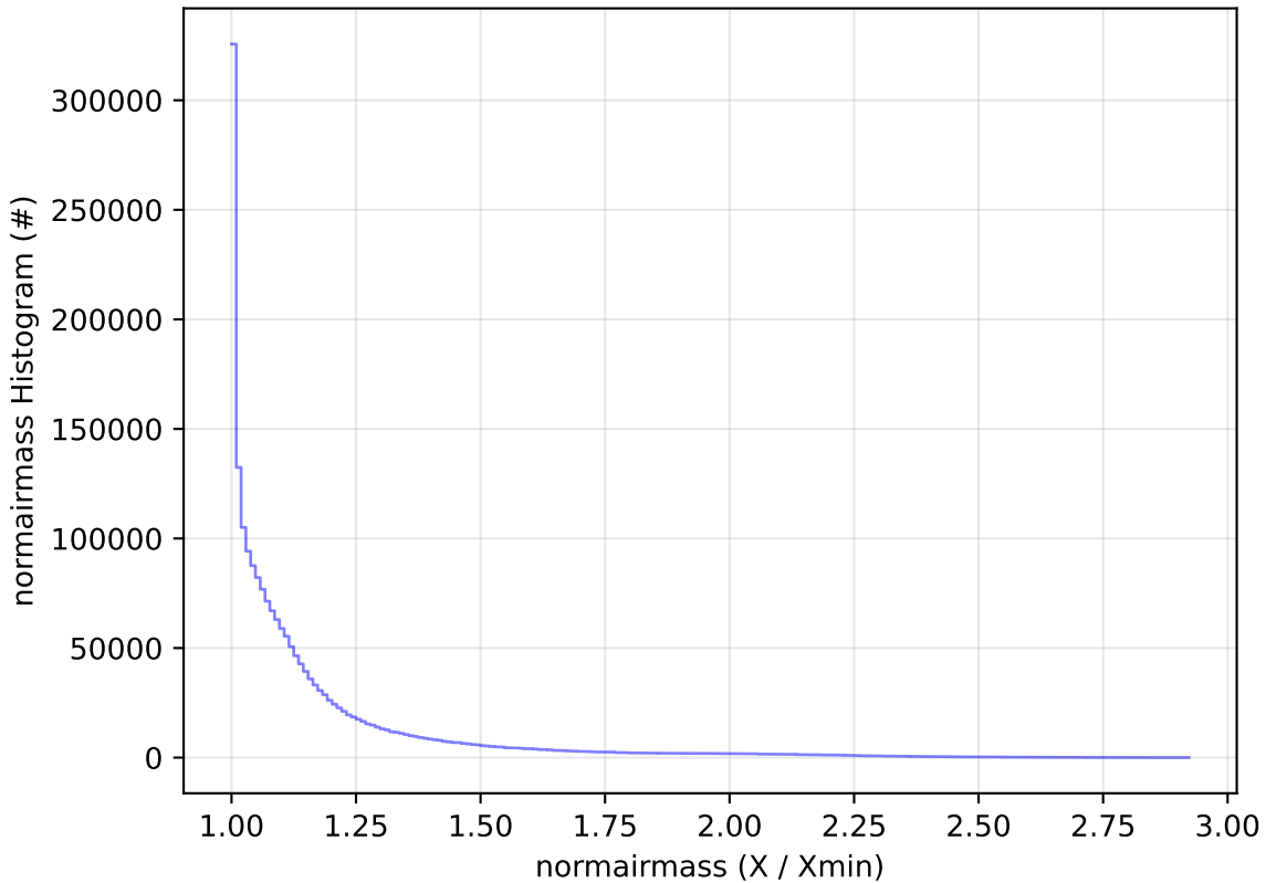
too_elab_r128_d3_ugrizy_v3.4_10yrs WFD all bands: normairmass Histogram
