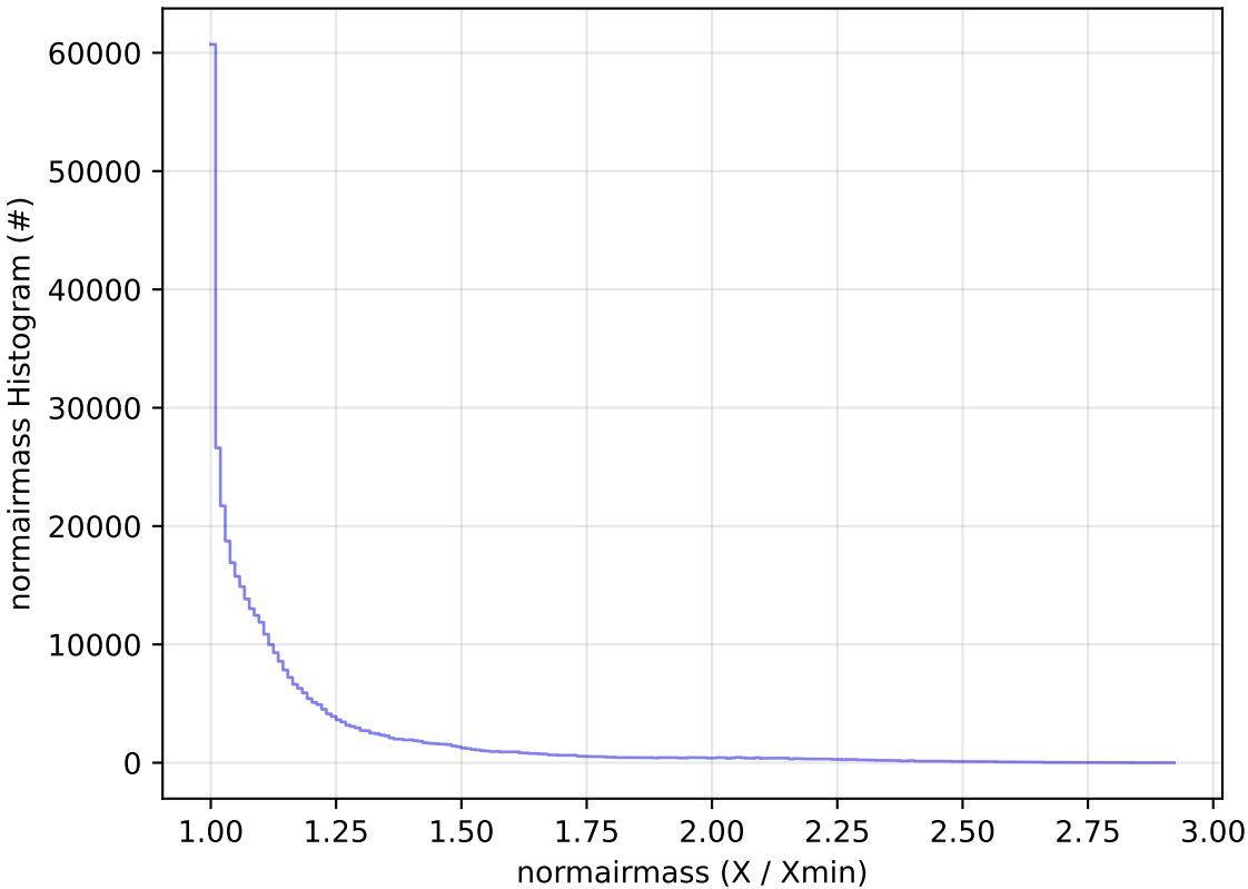
too_elab_r128_d3_ugrizy_v3.4_10yrs All sky z band: normairmass Histogram
