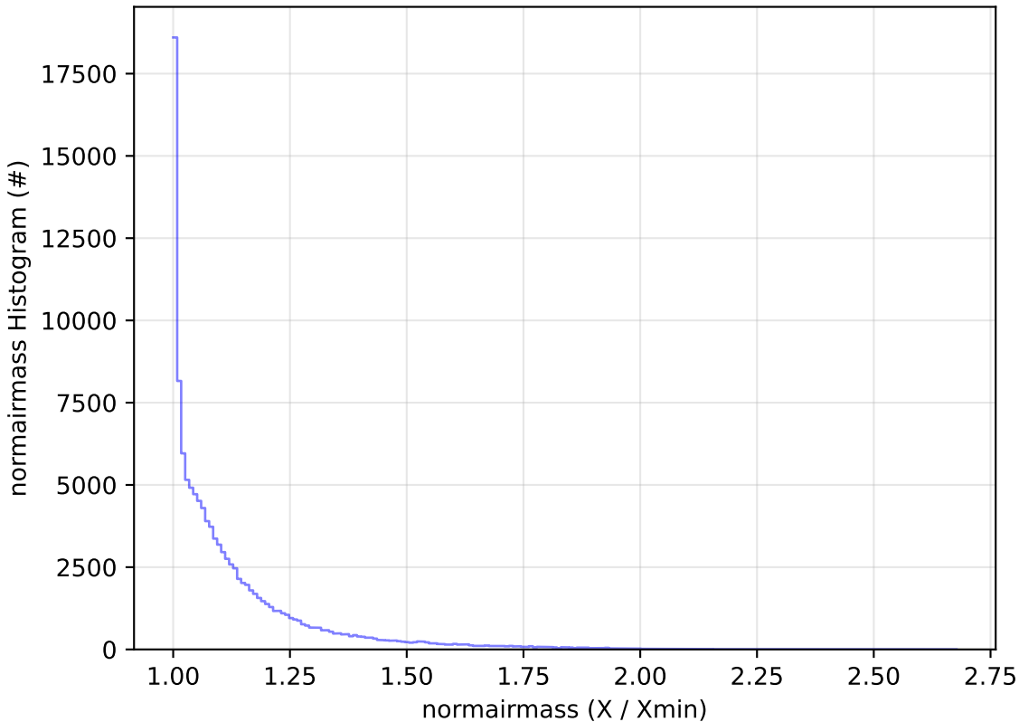
too_elab_r128_d3_ugrizy_v3.4_10yrs All sky u band: normairmass Histogram
