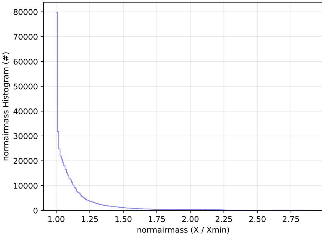
too_elab_r128_d3_ugrizy_v3.4_10yrs All sky r band: normairmass Histogram
