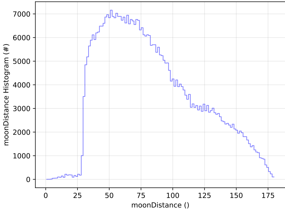
too_elab_r128_d3_ugrizy_v3.4_10yrs WFD z band: moonDistance Histogram
