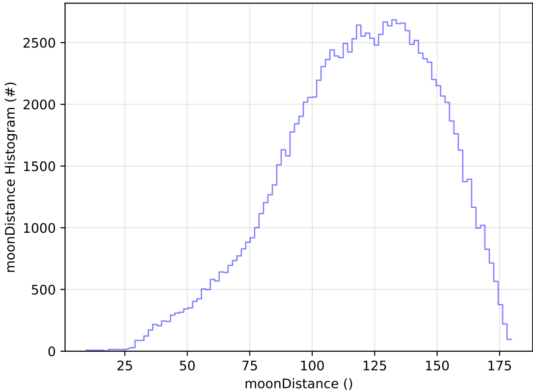
too_elab_r128_d3_ugrizy_v3.4_10yrs WFD u band: moonDistance Histogram
