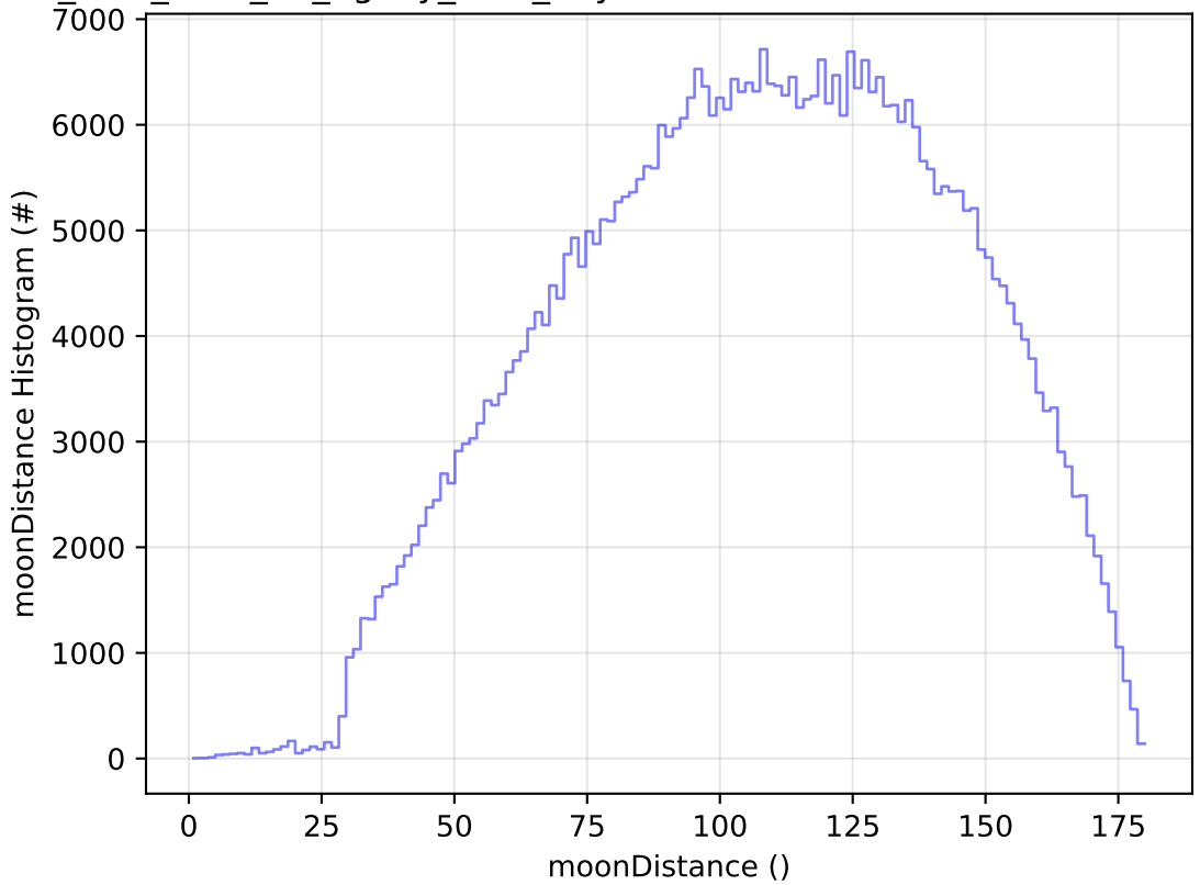
too_elab_r128_d3_ugrizy_v3.4_10yrs WFD r band: moonDistance Histogram
