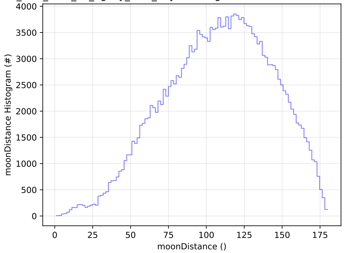
too_elab_r128_d3_ugrizy_v3.4_10yrs WFD g band: moonDistance Histogram
