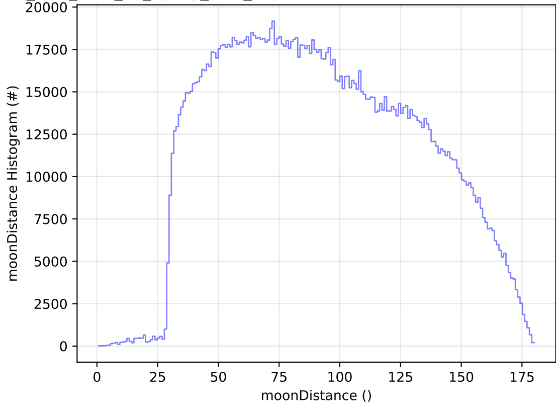
too_elab_r128_d3_ugrizy_v3.4_10yrs WFD all bands: moonDistance Histogram
