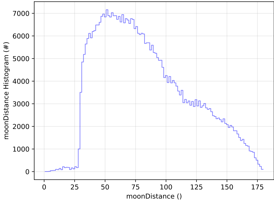
too_elab_r128_d3_ugrizy_v3.4_10yrs All sky z band: moonDistance Histogram
