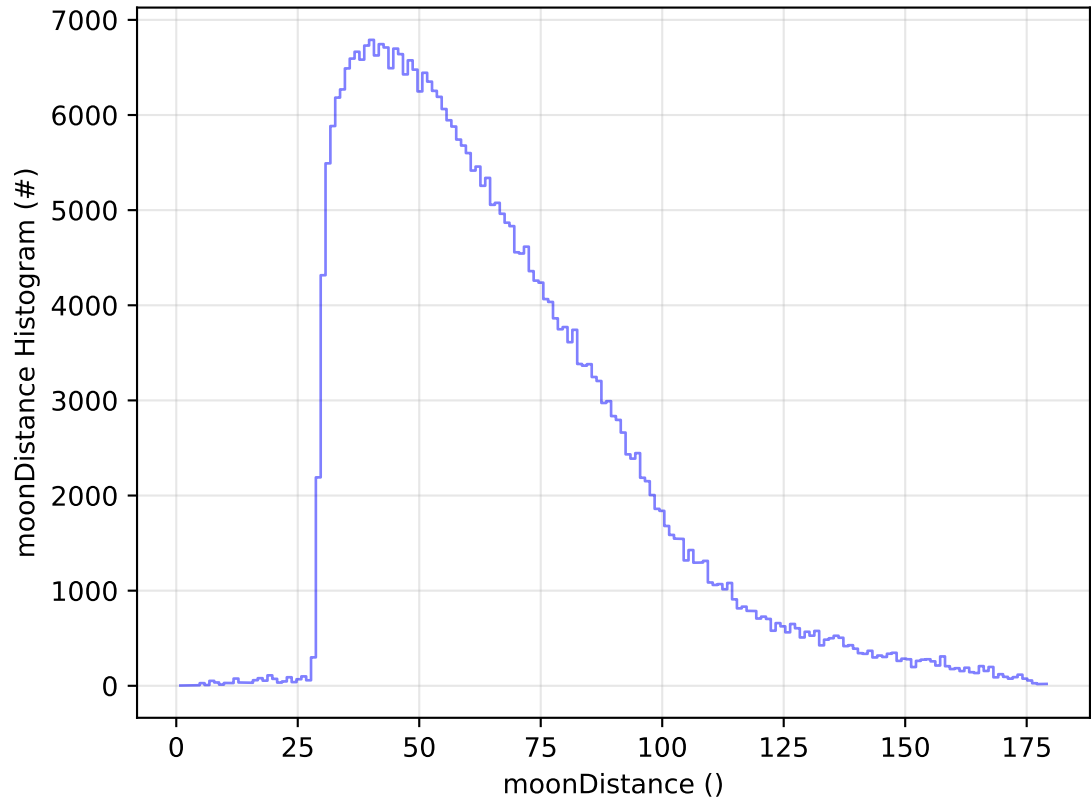
too_elab_r128_d3_ugrizy_v3.4_10yrs All sky y band: moonDistance Histogram
