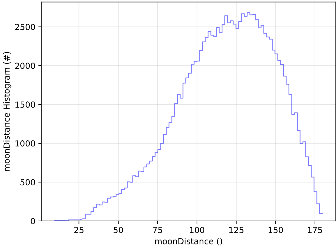
too_elab_r128_d3_ugrizy_v3.4_10yrs All sky u band: moonDistance Histogram
