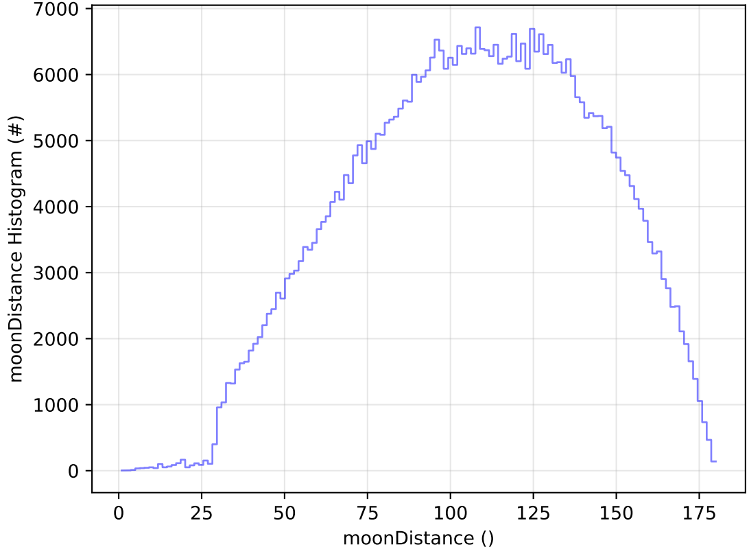
too_elab_r128_d3_ugrizy_v3.4_10yrs All sky r band: moonDistance Histogram
