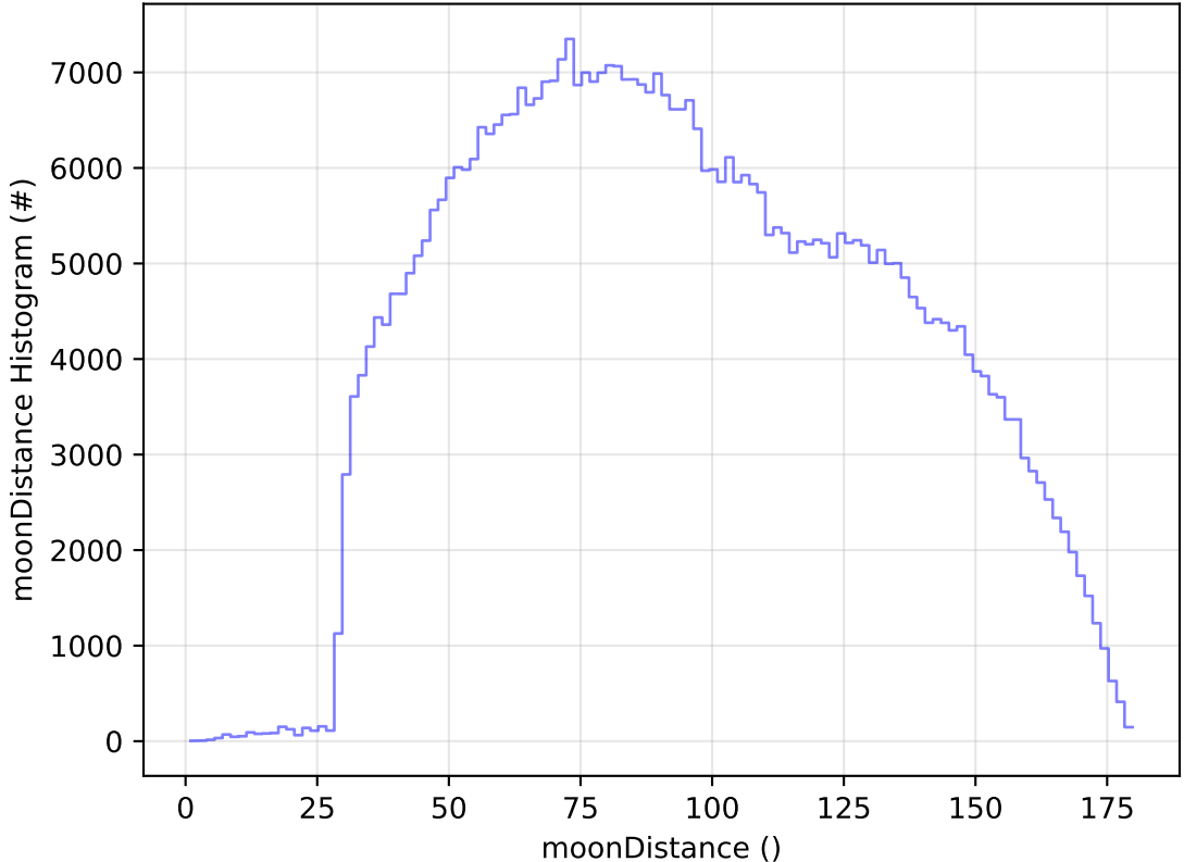
too_elab_r128_d3_ugrizy_v3.4_10yrs All sky i band: moonDistance Histogram
