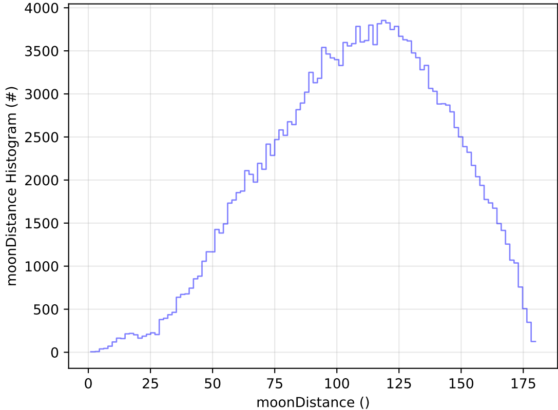
too_elab_r128_d3_ugrizy_v3.4_10yrs All sky g band: moonDistance Histogram
