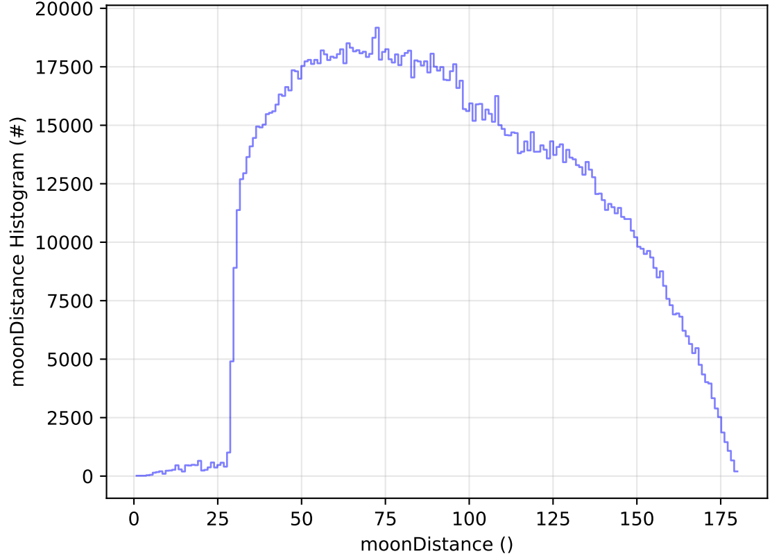
too_elab_r128_d3_ugrizy_v3.4_10yrs All sky all bands: moonDistance Histogram
