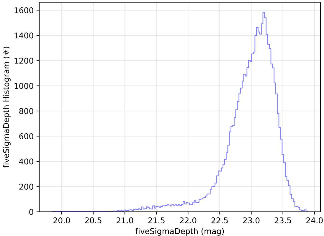
too_elab_r128_d3_ugrizy_v3.4_10yrs Yr 1 z band: fiveSigmaDepth Histogram
