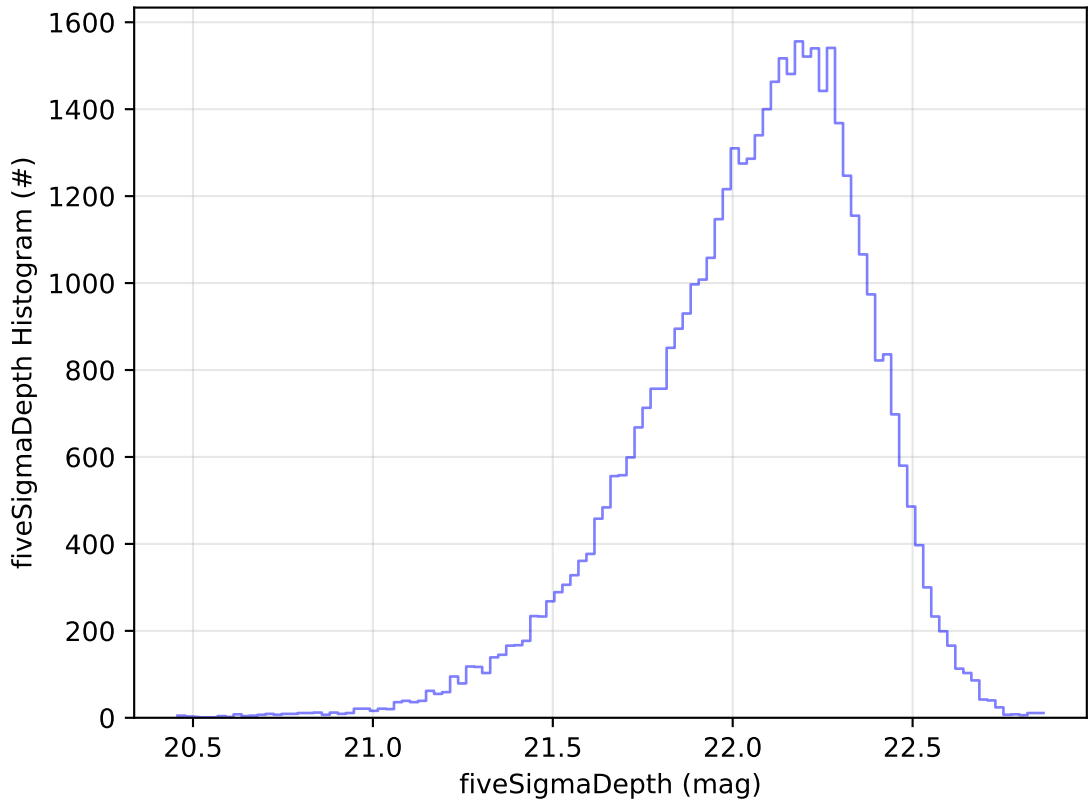
too_elab_r128_d3_ugrizy_v3.4_10yrs Yr 1 y band: fiveSigmaDepth Histogram
