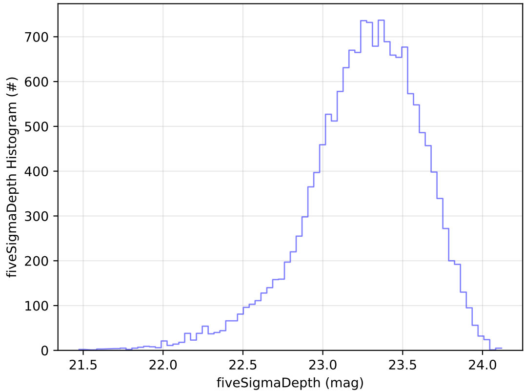
too_elab_r128_d3_ugrizy_v3.4_10yrs Yr 1 u band: fiveSigmaDepth Histogram
