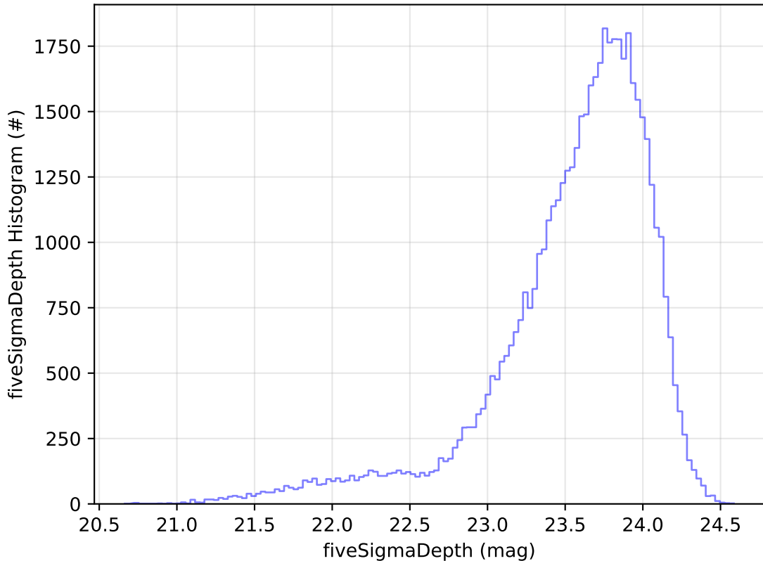
too_elab_r128_d3_ugrizy_v3.4_10yrs Yr 1 i band: fiveSigmaDepth Histogram
