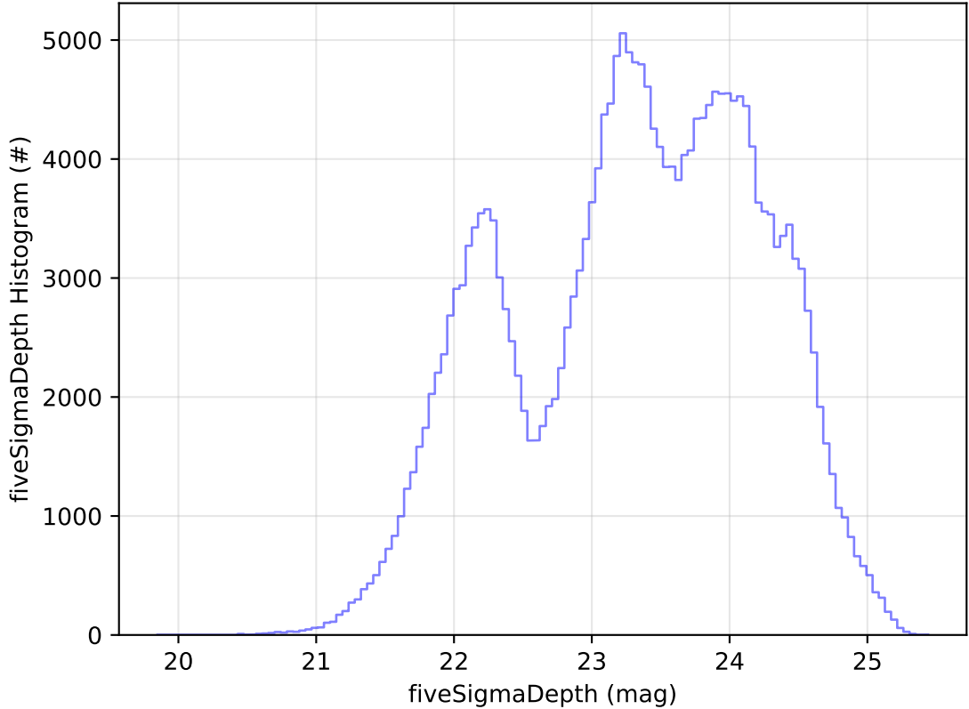
too_elab_r128_d3_ugrizy_v3.4_10yrs Yr 1 all bands: fiveSigmaDepth Histogram
