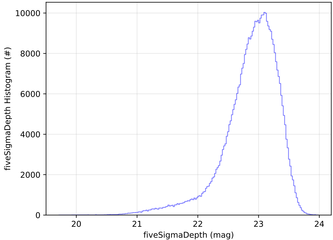
too_elab_r128_d3_ugrizy_v3.4_10yrs WFD z band: fiveSigmaDepth Histogram
