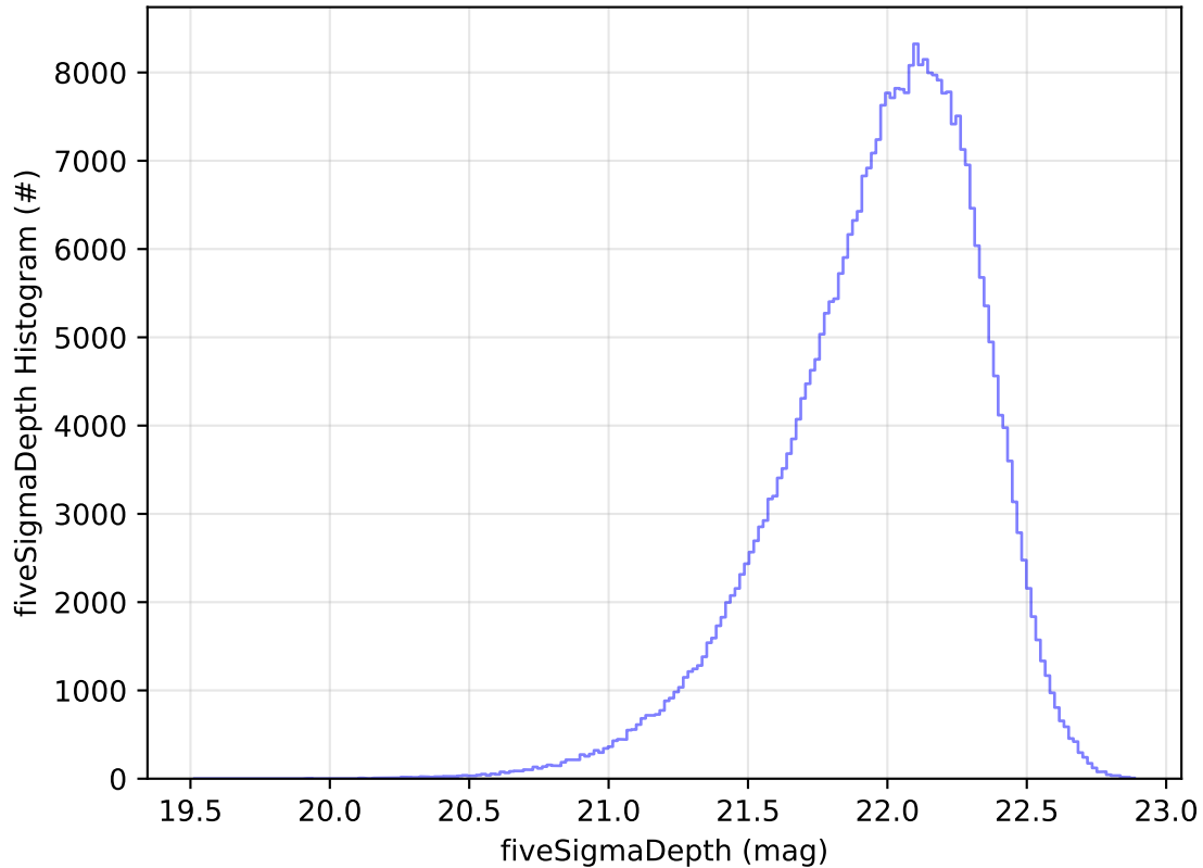
too_elab_r128_d3_ugrizy_v3.4_10yrs WFD y band: fiveSigmaDepth Histogram
