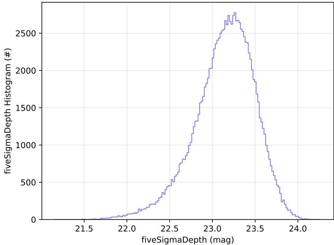
too_elab_r128_d3_ugrizy_v3.4_10yrs WFD u band: fiveSigmaDepth Histogram
