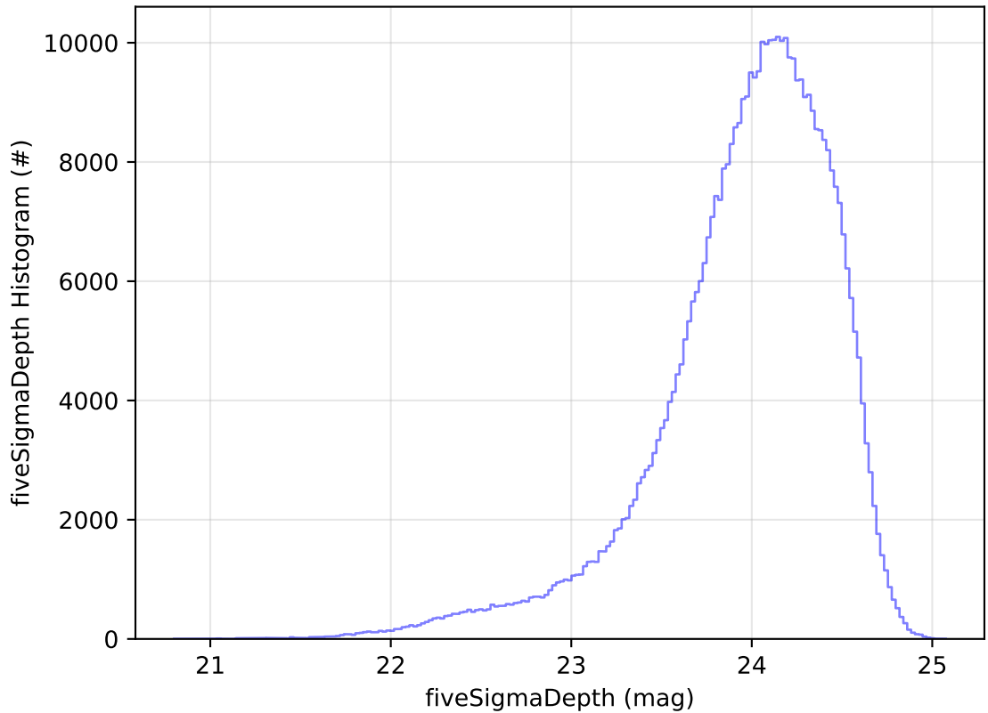
too_elab_r128_d3_ugrizy_v3.4_10yrs WFD r band: fiveSigmaDepth Histogram
