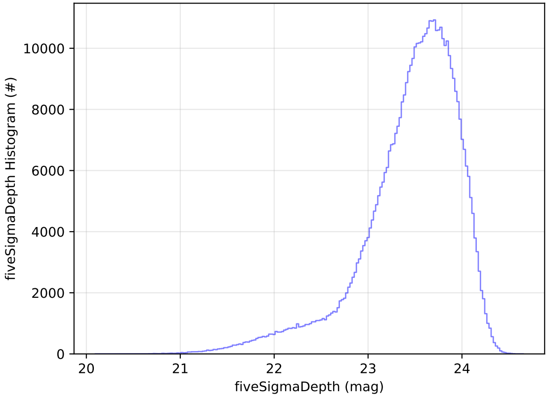
too_elab_r128_d3_ugrizy_v3.4_10yrs WFD i band: fiveSigmaDepth Histogram
