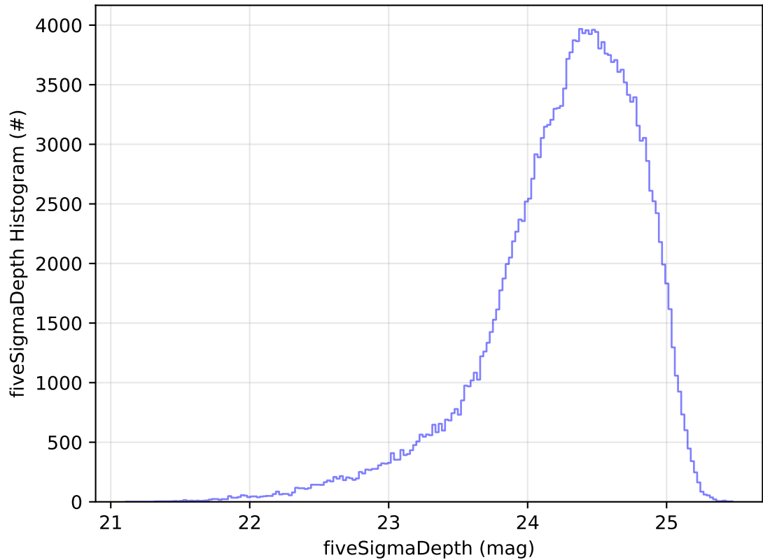
too_elab_r128_d3_ugrizy_v3.4_10yrs WFD g band: fiveSigmaDepth Histogram
