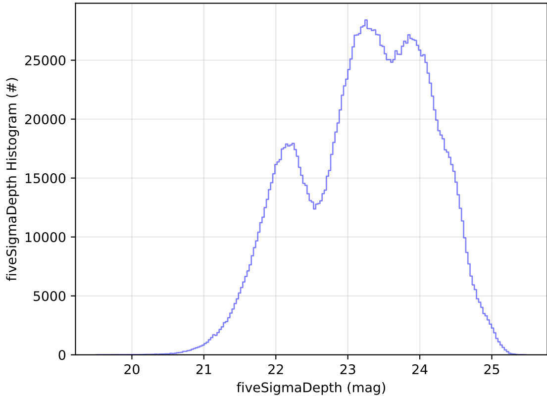
too_elab_r128_d3_ugrizy_v3.4_10yrs WFD all bands: fiveSigmaDepth Histogram
