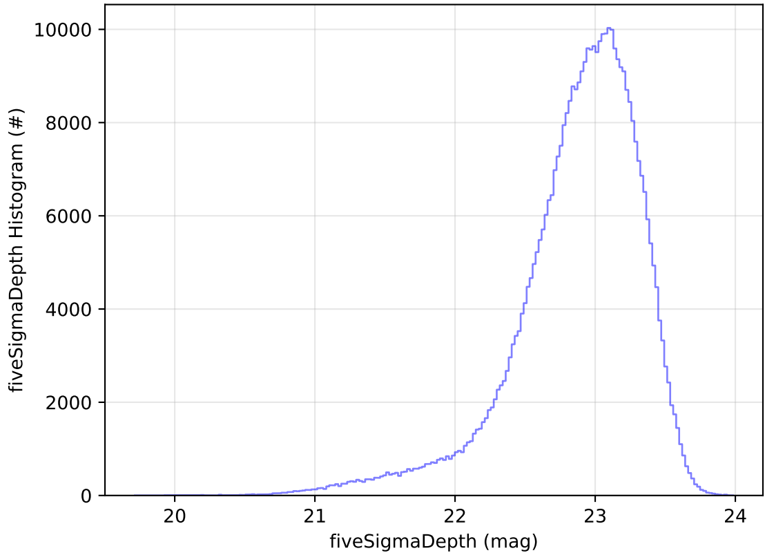
too_elab_r128_d3_ugrizy_v3.4_10yrs All sky z band: fiveSigmaDepth Histogram
