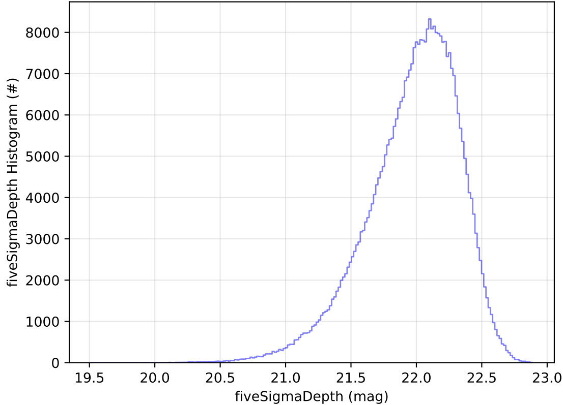
too_elab_r128_d3_ugrizy_v3.4_10yrs All sky y band: fiveSigmaDepth Histogram
