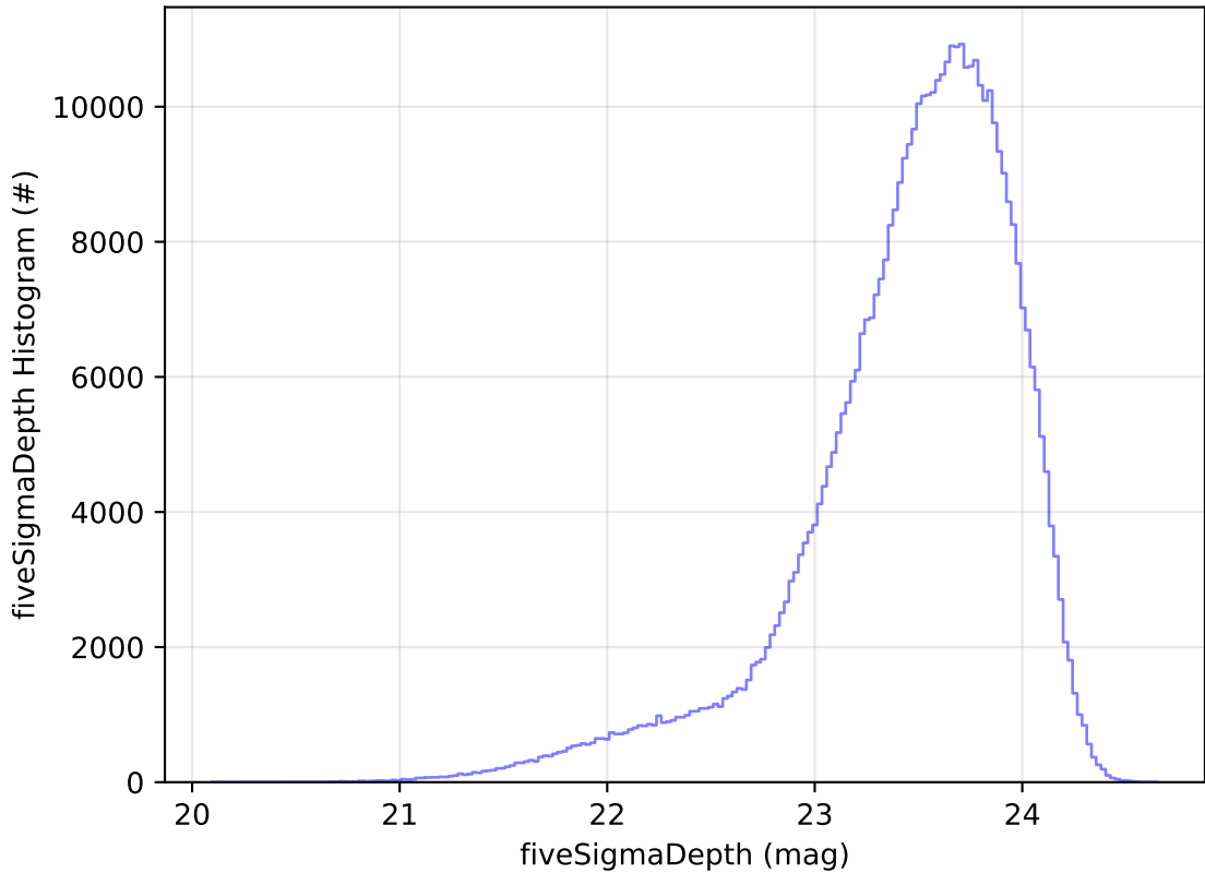
too_elab_r128_d3_ugrizy_v3.4_10yrs All sky i band: fiveSigmaDepth Histogram
