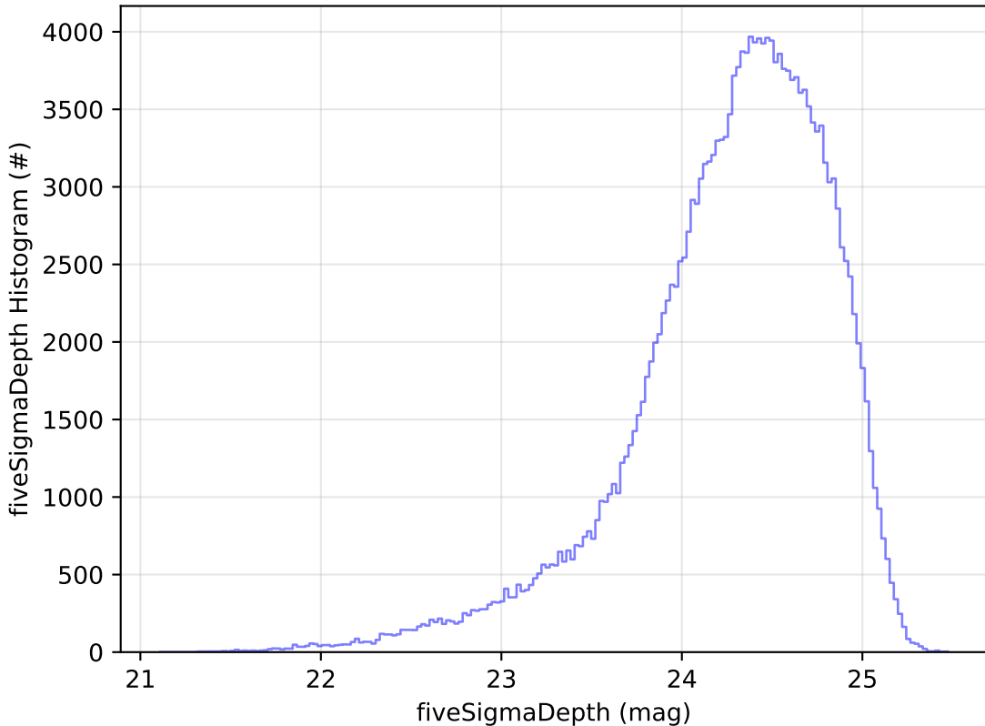
too_elab_r128_d3_ugrizy_v3.4_10yrs All sky g band: fiveSigmaDepth Histogram
