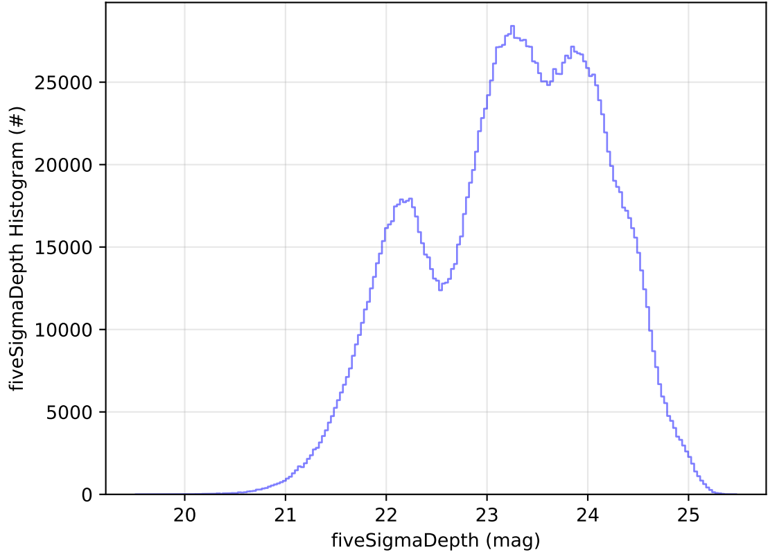
too_elab_r128_d3_ugrizy_v3.4_10yrs All sky all bands: fiveSigmaDepth Histogram
