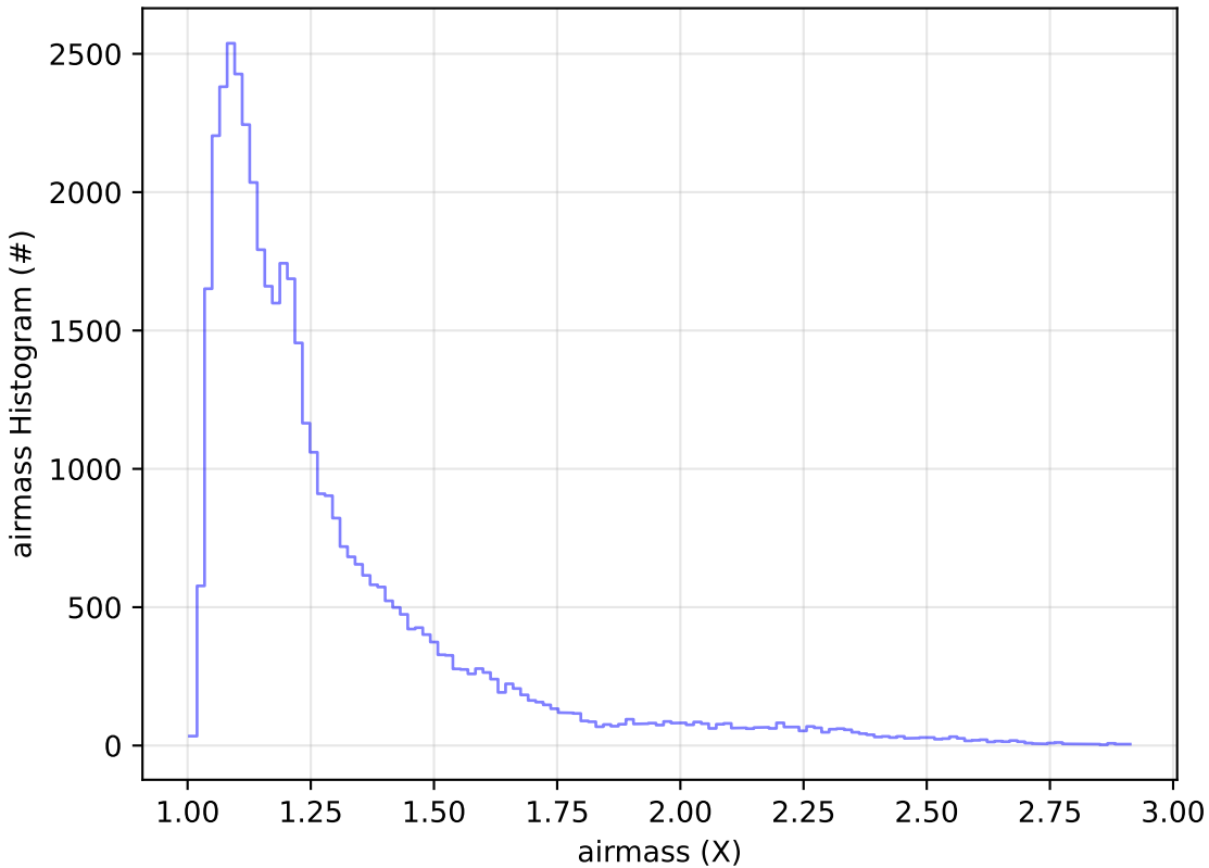
too_elab_r128_d3_ugrizy_v3.4_10yrs Yr 1 z band: airmass Histogram
