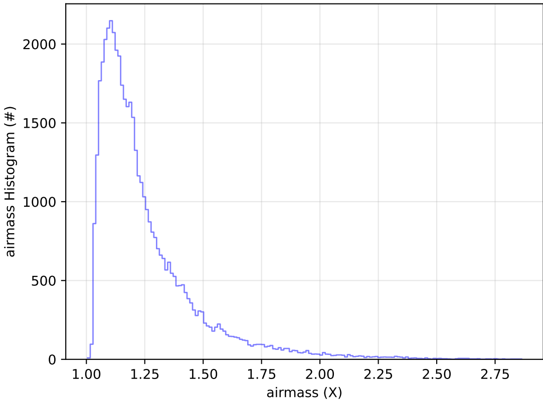
too_elab_r128_d3_ugrizy_v3.4_10yrs Yr 1 y band: airmass Histogram
