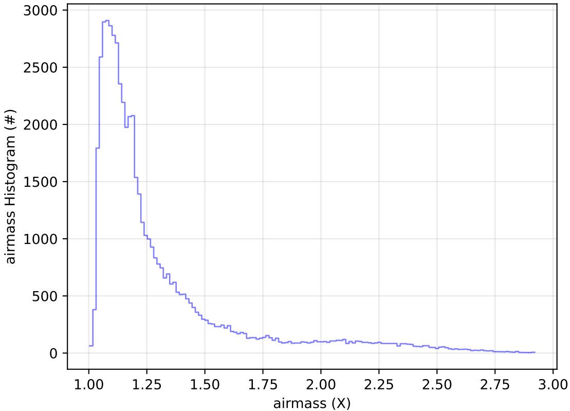
too_elab_r128_d3_ugrizy_v3.4_10yrs Yr 1 i band: airmass Histogram
