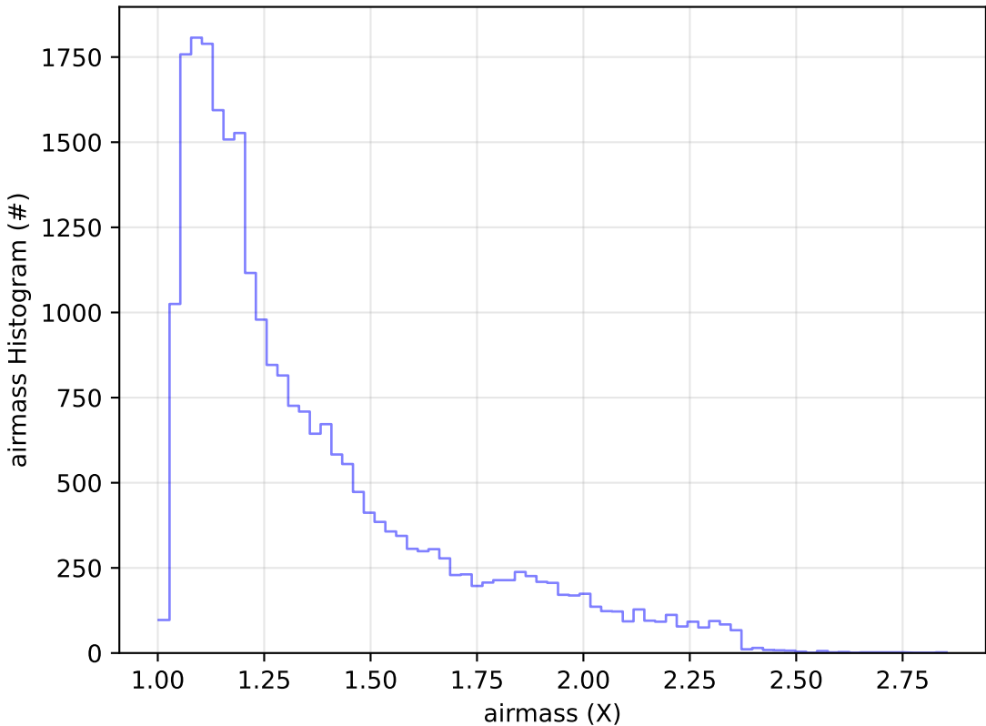
too_elab_r128_d3_ugrizy_v3.4_10yrs Yr 1 g band: airmass Histogram
