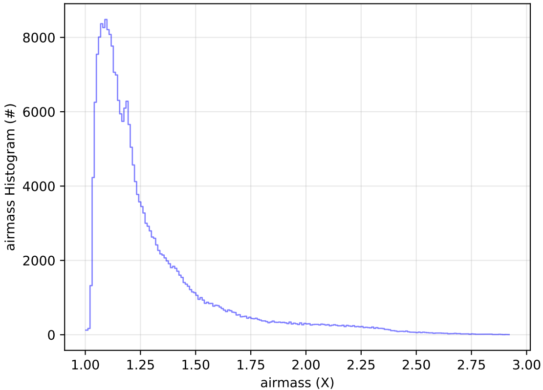
too_elab_r128_d3_ugrizy_v3.4_10yrs Yr 1 all bands: airmass Histogram
