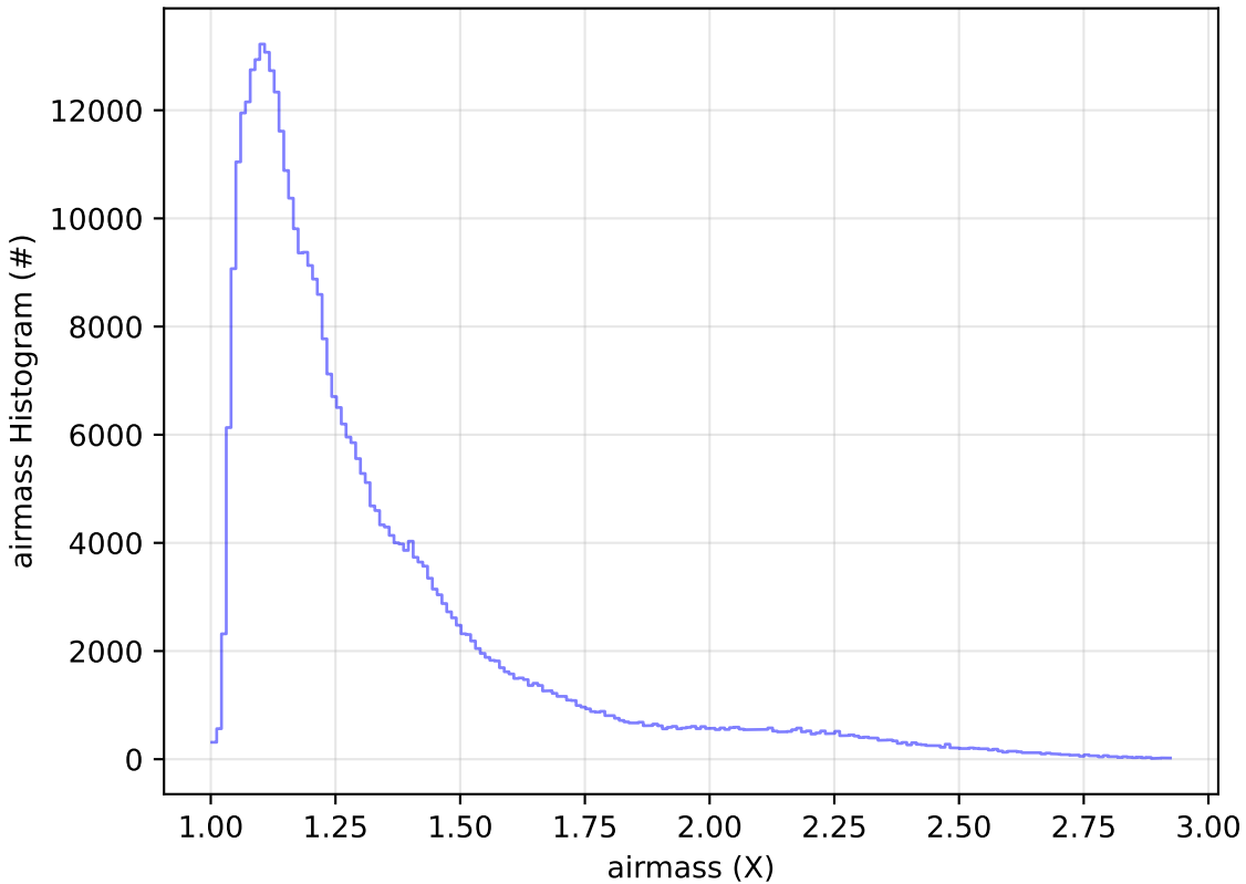
too_elab_r128_d3_ugrizy_v3.4_10yrs WFD z band: airmass Histogram
