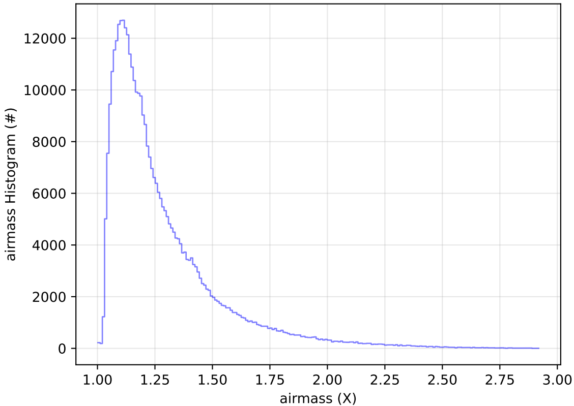
too_elab_r128_d3_ugrizy_v3.4_10yrs WFD y band: airmass Histogram
