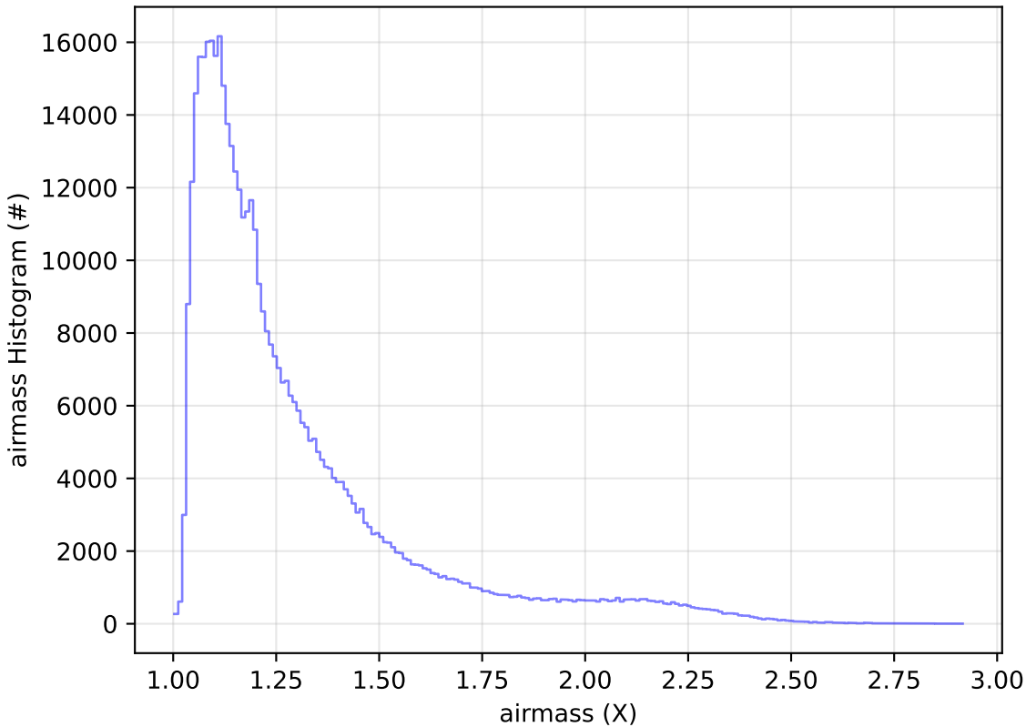
too_elab_r128_d3_ugrizy_v3.4_10yrs WFD r band: airmass Histogram
