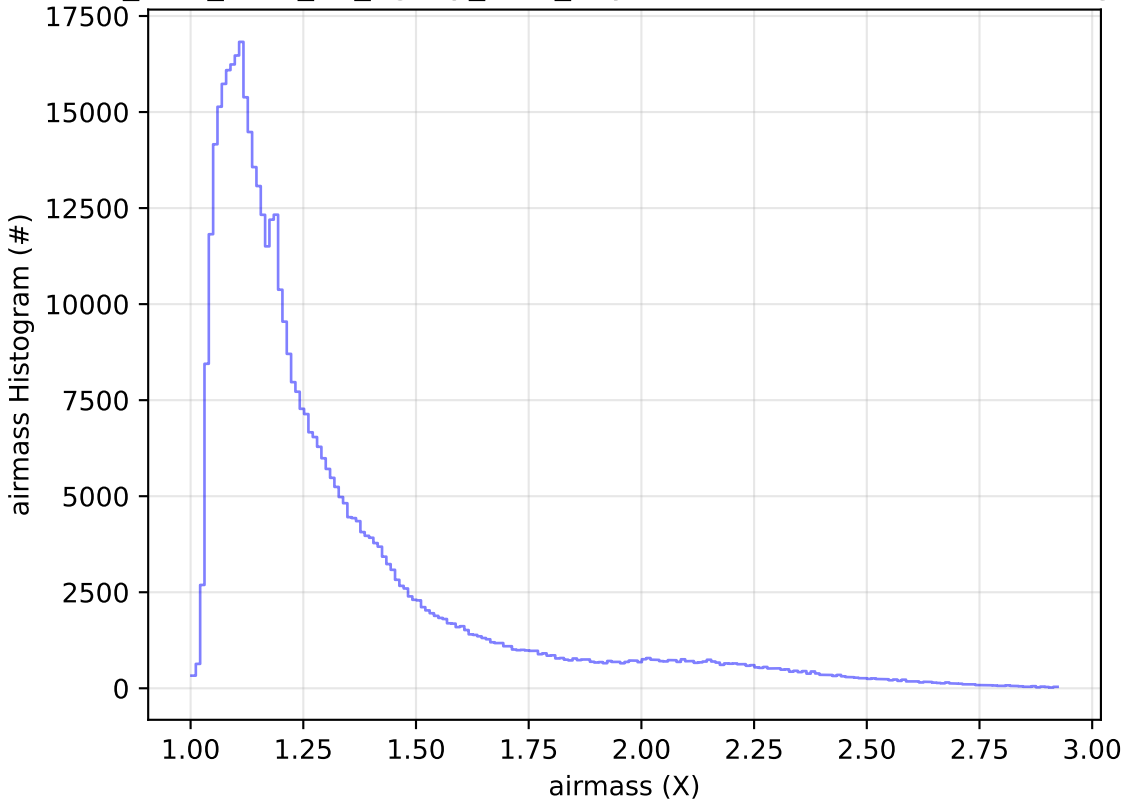
too_elab_r128_d3_ugrizy_v3.4_10yrs WFD i band: airmass Histogram
