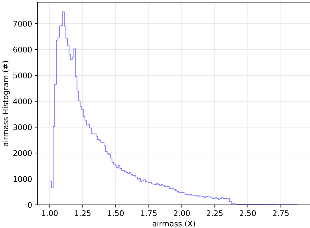
too_elab_r128_d3_ugrizy_v3.4_10yrs WFD g band: airmass Histogram
