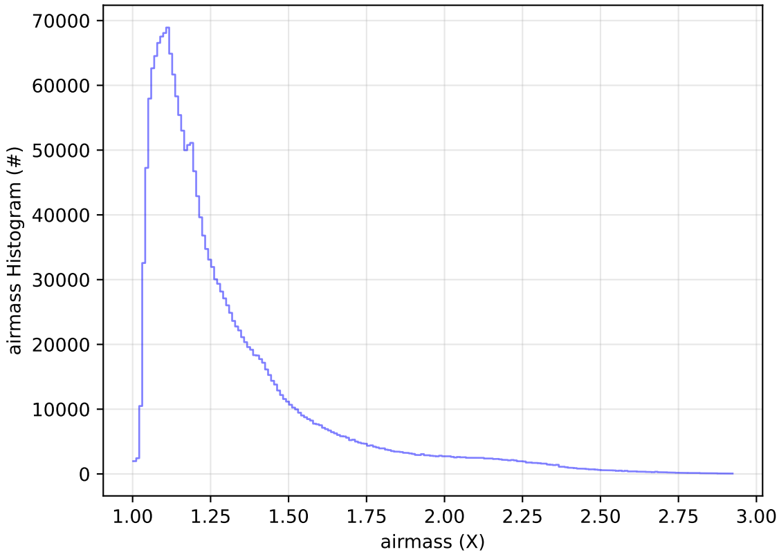
too_elab_r128_d3_ugrizy_v3.4_10yrs WFD all bands: airmass Histogram
